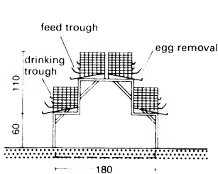
④ Aviary system
